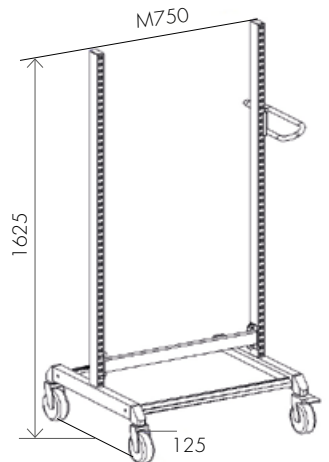
Basic trolley frame
